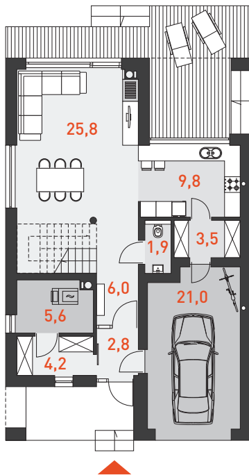
RZUT PARTERU 54,0 m 2
